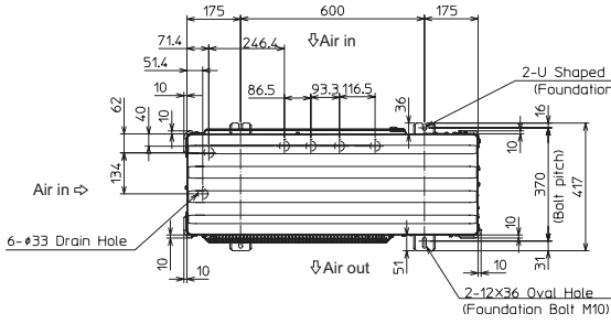
MXZ-5E102VA
